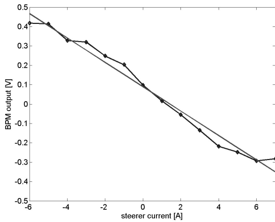
Figure 5: Vertical movement by a steerer magnet 5 m upstream the BPM. Outside this range beam loss occurred.
