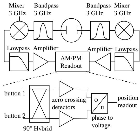
Figure 1: Block diagram of the BPM readout.
