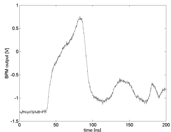
Figure 4: Beam Position Signal.
