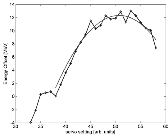
Figure 6: Energy variation by adjusting two acceleration sections of the linac. The nominal setting is 45.
