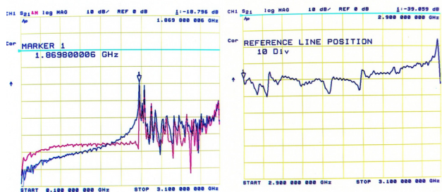
Figure 2: Frequency Response of the BPM.
