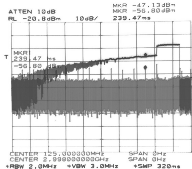
Figure 3: Frequency selected response of a single button, photographed from a spectrum analyzer in zero span mode. Two frequencies are shown, 125 MHz and 3 GHz.
